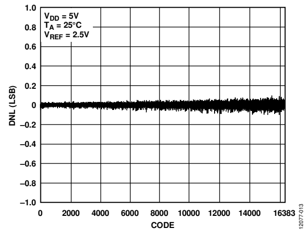
Figure 13. AD5692R DNL
