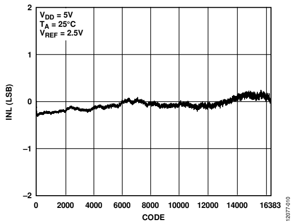
Figure 10. AD5692R INL
