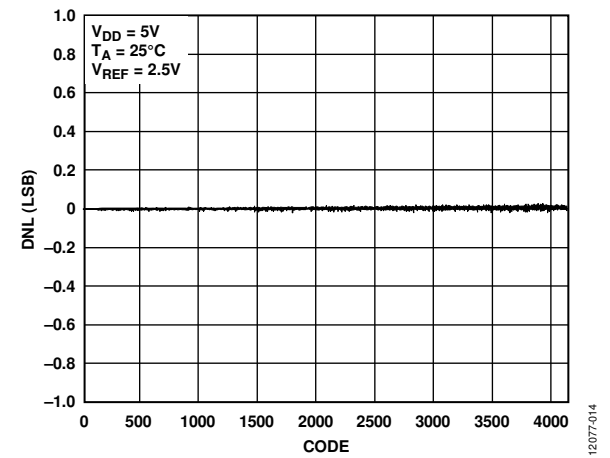
Figure 14. AD5691R DNL
