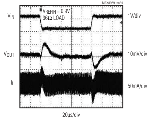
LINE TRANSIENT 4.2V TO 3.2V TO 4.2V
