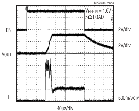
ENABLE WAVEFORMS
