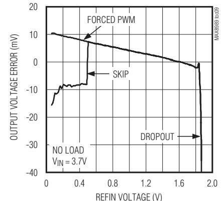
OUTPUT VOLTAGE ERROR vs. REFIN VOLTAGE
