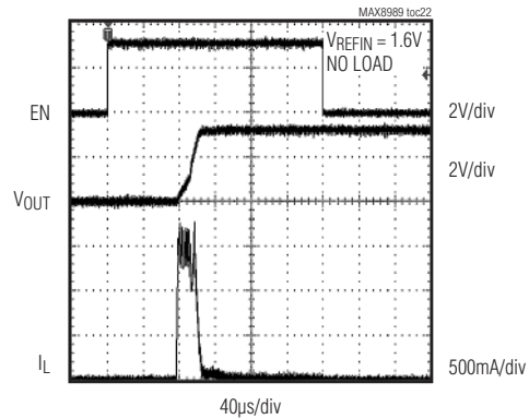
ENABLE WAVEFORMS
