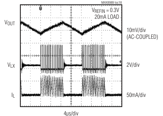
LIGHT-LOAD SWITCHING WAVEFORMS (SKIP)
