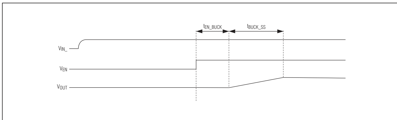
Figure 2. Power-Up Timing
