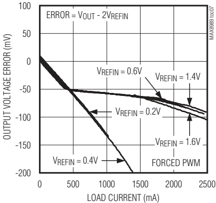
LOAD REGULATION ERROR vs. LOAD CURRENT
