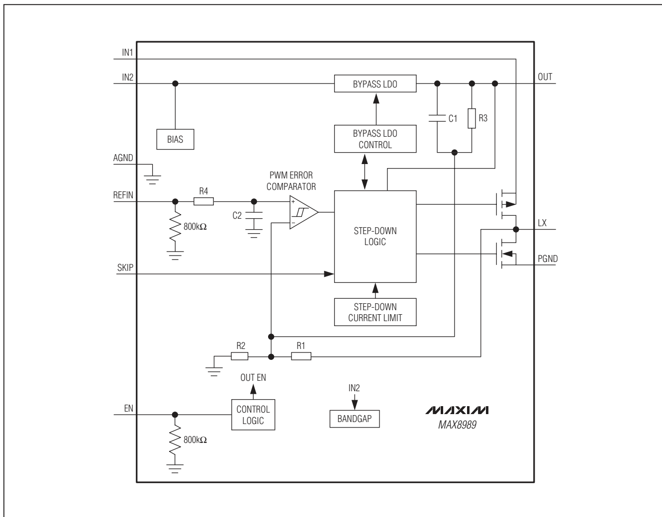
Figure 1. Functional Diagram
