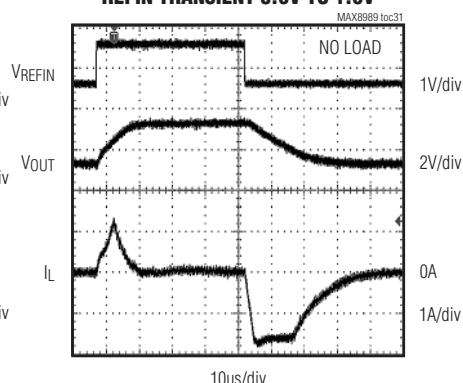
REFIN TRANSIENT 0.6V TO 1.6V
