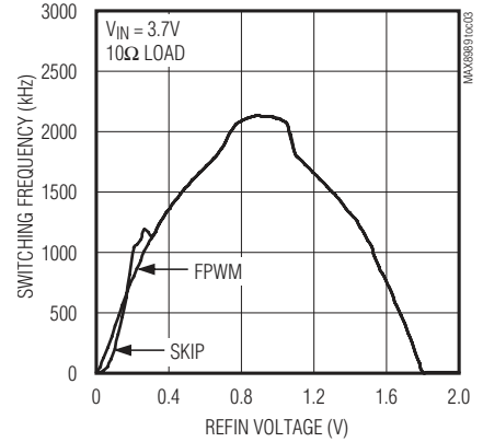
SWITCHING FREQUENCY vs. REFIN VOLTAGE
