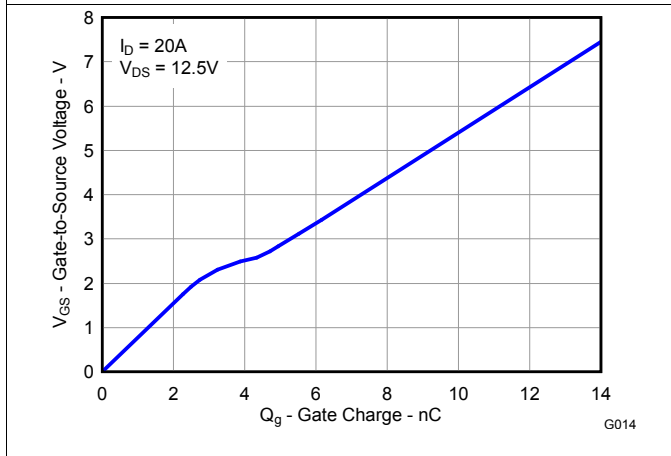
Figure 14. Control MOSFET Gate Charge
