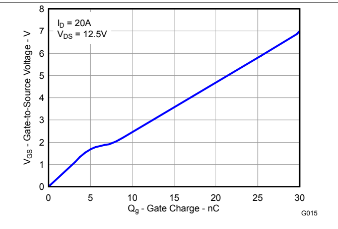
Figure 15. Sync MOSFET Gate Charge
