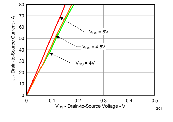
Figure 11. Sync MOSFET Saturation
