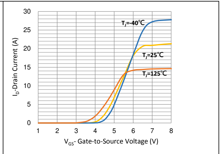
Fig.2 Transfer Characteristics
