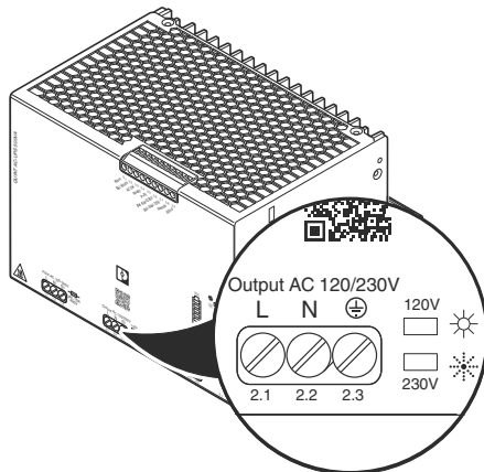
Figure 11 Output voltage connection terminal blocks: Output AC L/N/⊕ (2.1...2.3)
