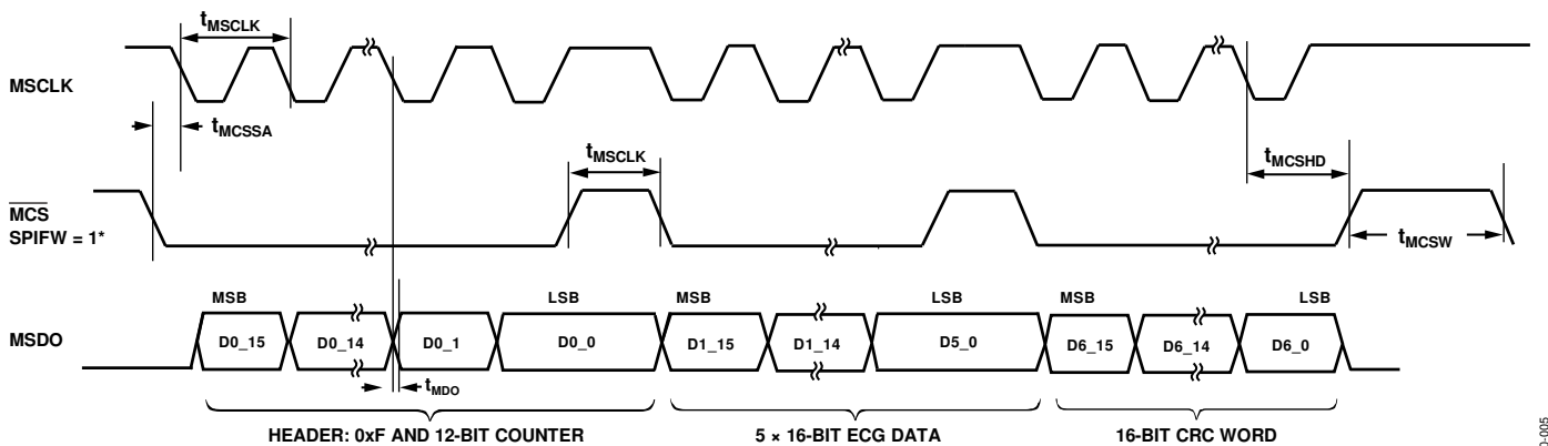
*SPIFW = 1 PROVIDES \overline{MCS} FOR EACH FRAME, SCLK STAYS HIGH FOR 1 MSCLK CYCLE BETWEEN EACH WORD.
