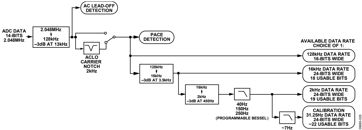
Figure 75. ECG Channel Filter Signal Flow
