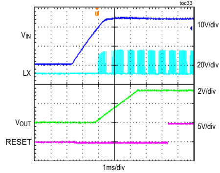
STARTUP THROUGH INPUT SUPPLY V_{IN} = 24V, V_{OUT} = 3.3V, I_{OUT} = 2.5A, MODE = SGND
