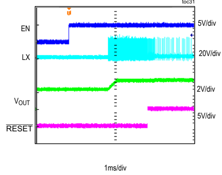
STARTUP WITH 2.5V PREBIAS V_{IN} = 24V, V_{OUT} = 3.3V, I_{OUT} = 0A, MODE = OPEN
