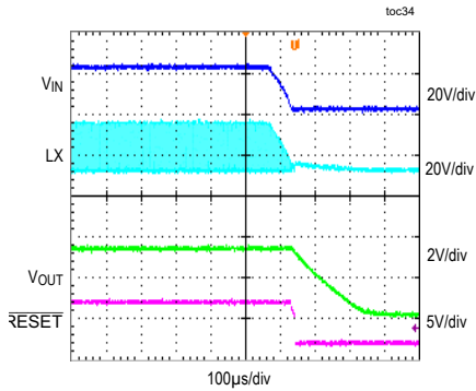
SHUTDOWN THROUGH INPUT SUPPLY V_{IN} = 24V, V_{OUT} = 3.3V, I_{OUT} = 2.5A, MODE = SGND
