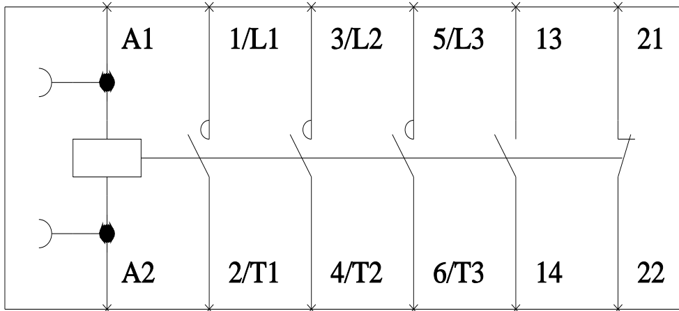
LENO0C003 Wiring Diagram
