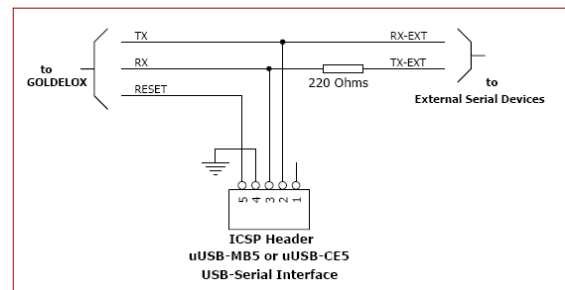
ICSP Interface
