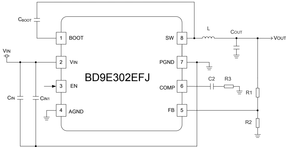
Figure 56. Application Circuit 3
