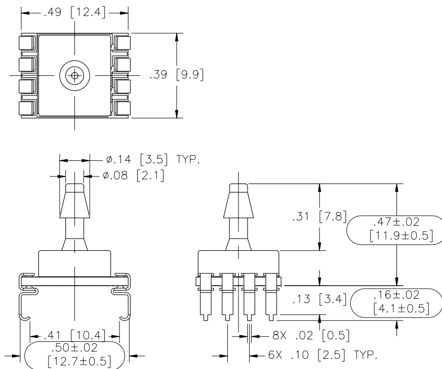
Model: MS4525DO-TPvoixxyS
