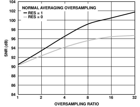
Figure 20. SNR vs. Oversampling Ratio, Normal Averaging
