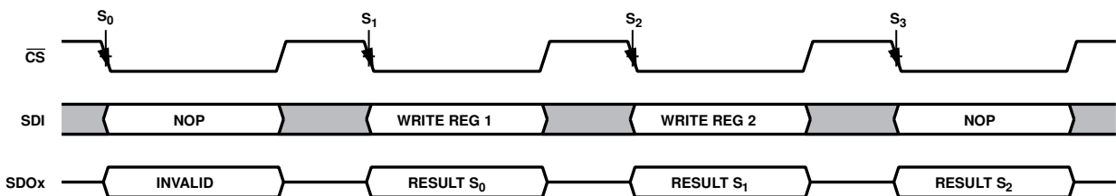
Figure 41. Register Write
