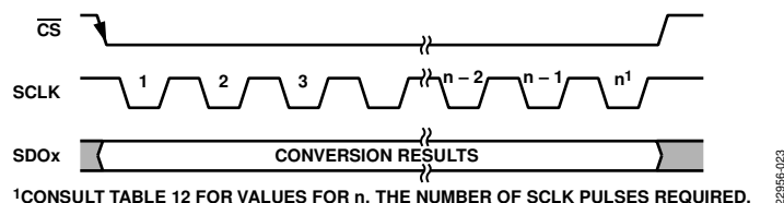
Figure 35. Reading Conversion Results
