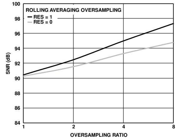
Figure 21. SNR vs. Oversampling Ratio, Rolling Average
