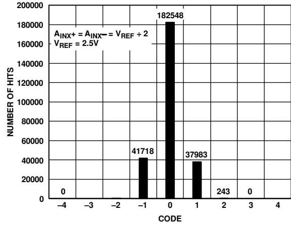
Figure 24. DC Histogram Codes at Code Center
