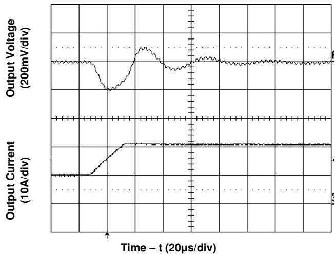
Figure 11. Transient Load Response (typical V_{in} , load current steps from 50% to 100% at a slew rate 0.5A/µs)
