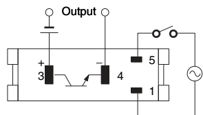
G3TA-IAZR02S
