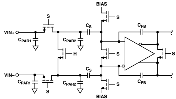
Figure 43. Switched Capacitor Input
