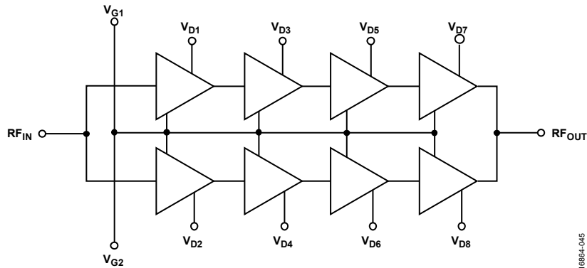
Figure 48. Simplified Schematic Diagram of Amplifier Stages
