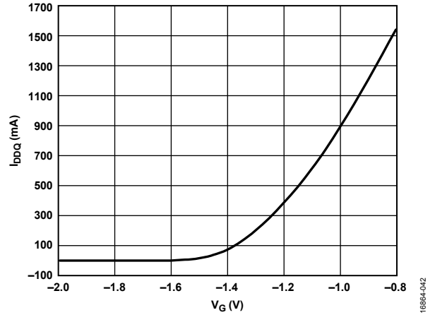
Figure 47. I_{DDQ} vs. Gate Bias Voltage ( V_G ), V_{DX} = 5.5 V, Representative of a Typical Device
