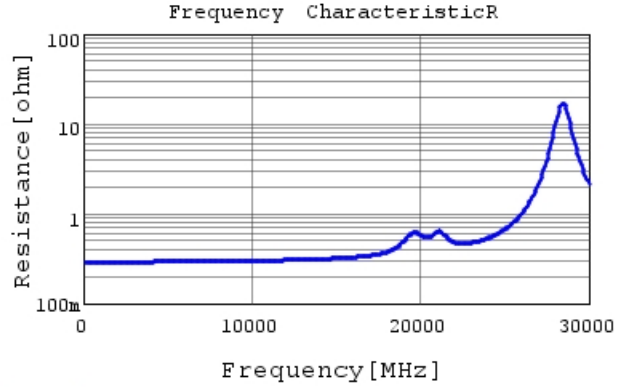
GJM0335C1E1R2CB01 R DC0V, 25degC
