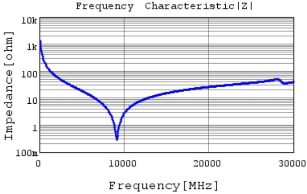
GJM0335C1E1R2CB01 |Z| DC0V, 25degC
