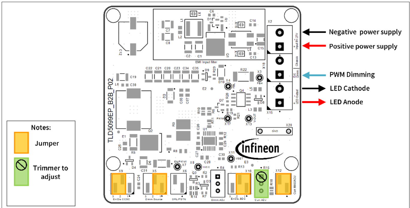
Figure 4 Current adjustment
