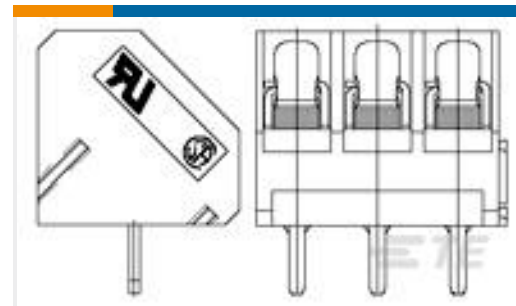
TE Part #1776252-6 45 degree wire inlet, 5.0mm, H
