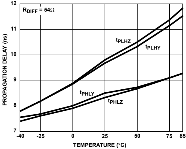
FIGURE 13. DRIVER PROPAGATION DELAY vs TEMPERATURE
