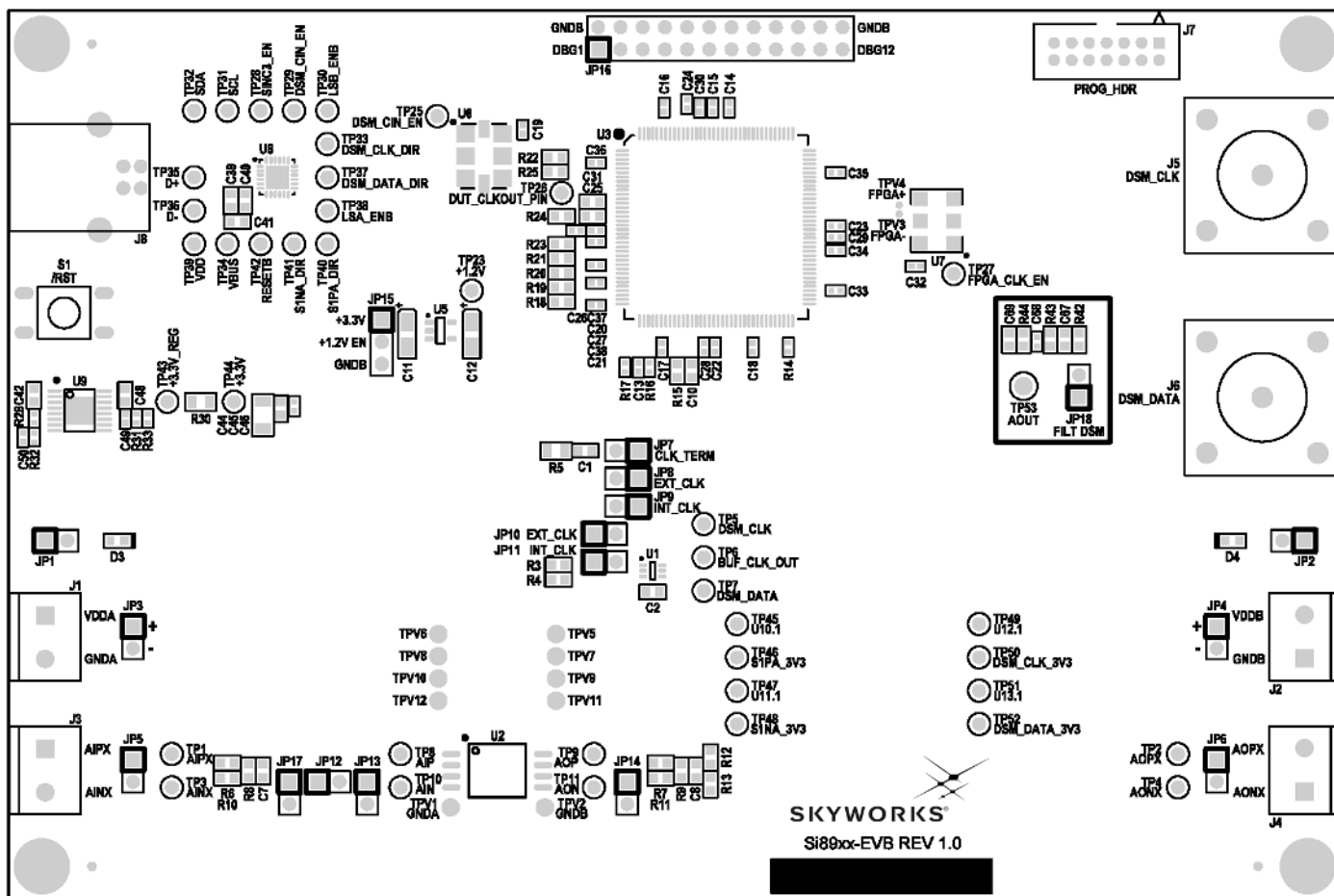
Figure 2.2. Primary Silkscreen
