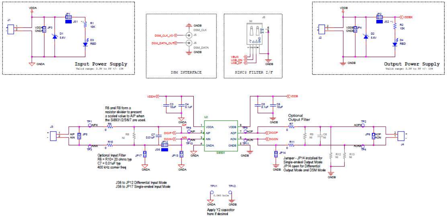
Figure 2.8. Top Level
