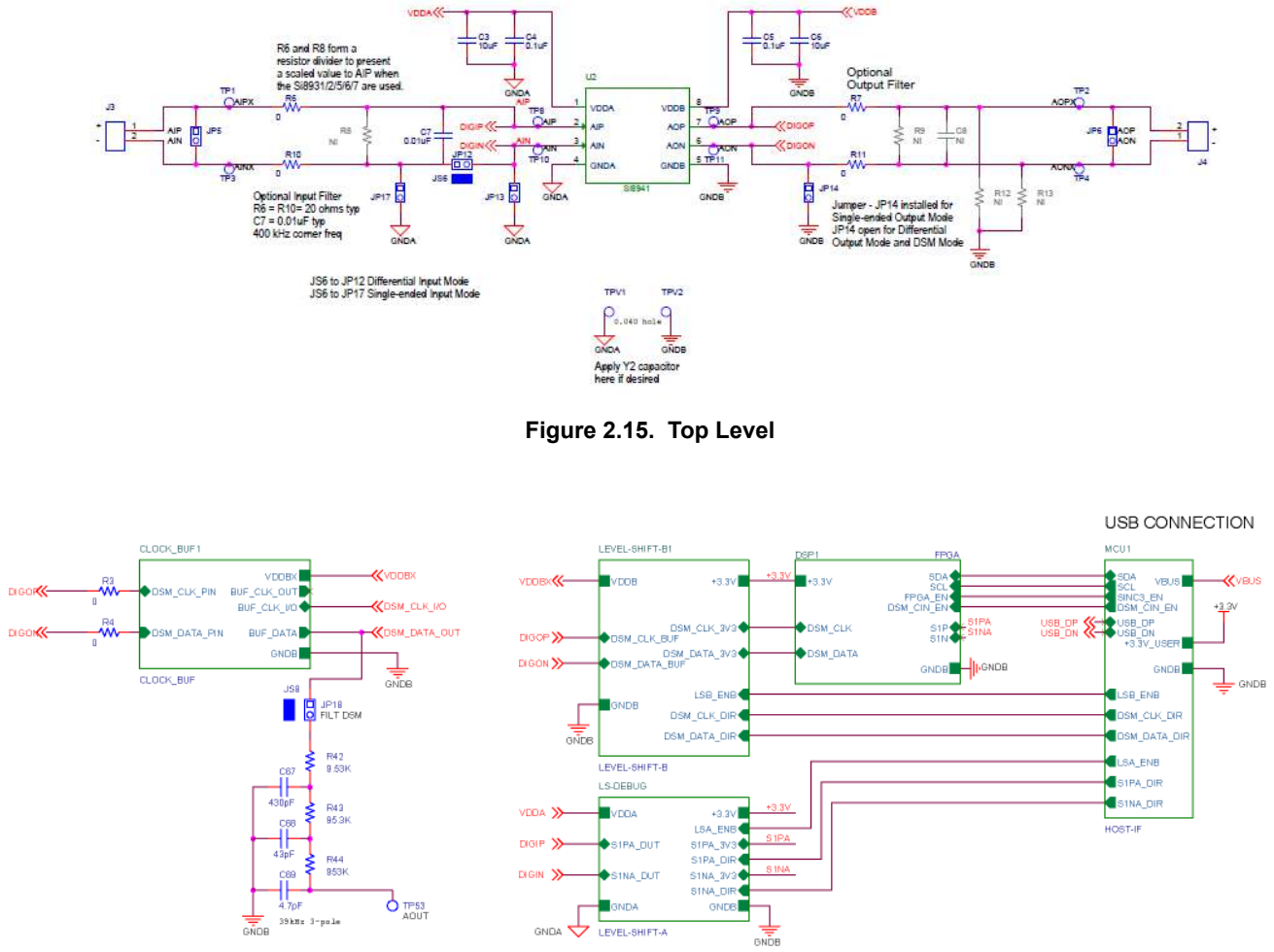
Figure 2.16. Digital
