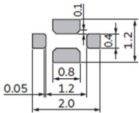
NFM18PS
