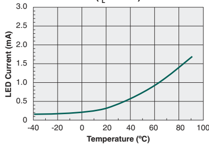
Typical I_F for Switch Operation vs. Temperature ( I_L=60mA )
