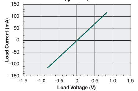
Typical Load Current vs. Load Voltage ( I_F=1mA )
