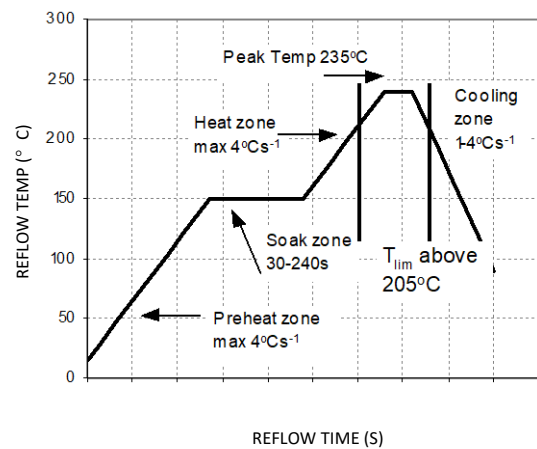
Figure 37. Reflow Profile for Tin/Lead (Sn/Pb) process.
