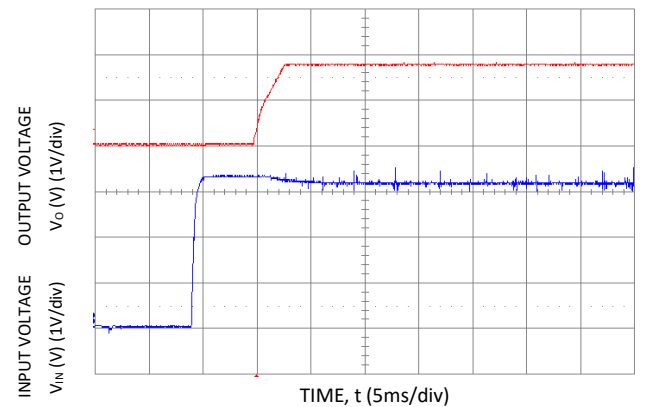
Figure 18. Typical Start-up Using Input Voltage ( V_{IN} = V_{IN,NOM} , I_o = I_{o,max} ).
