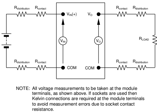
Figure 27. Output Voltage and Efficiency Test Setup.
