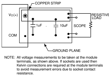
Figure 26. Output Ripple and Noise Test Setup.
