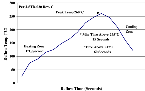
Figure 39. Recommended linear reflow profile using Sn/Ag/Cu solder.
