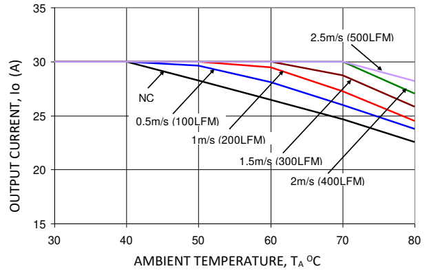
Figure 23. Output Current Derating versus Ambient Temperature and Airflow (ATM030A0X3-SRH).
