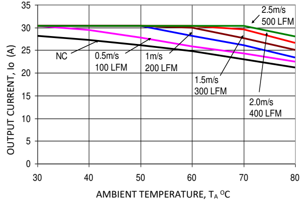
Figure 10. Derating Output Current versus Ambient Temperature and Airflow (ATM030A0X3-SR).
