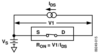
Figure 3. On Resistance
