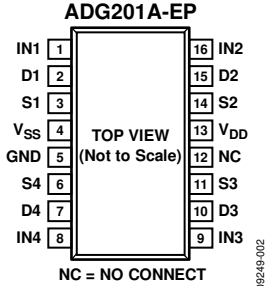
Figure 2. Pin Configuration
