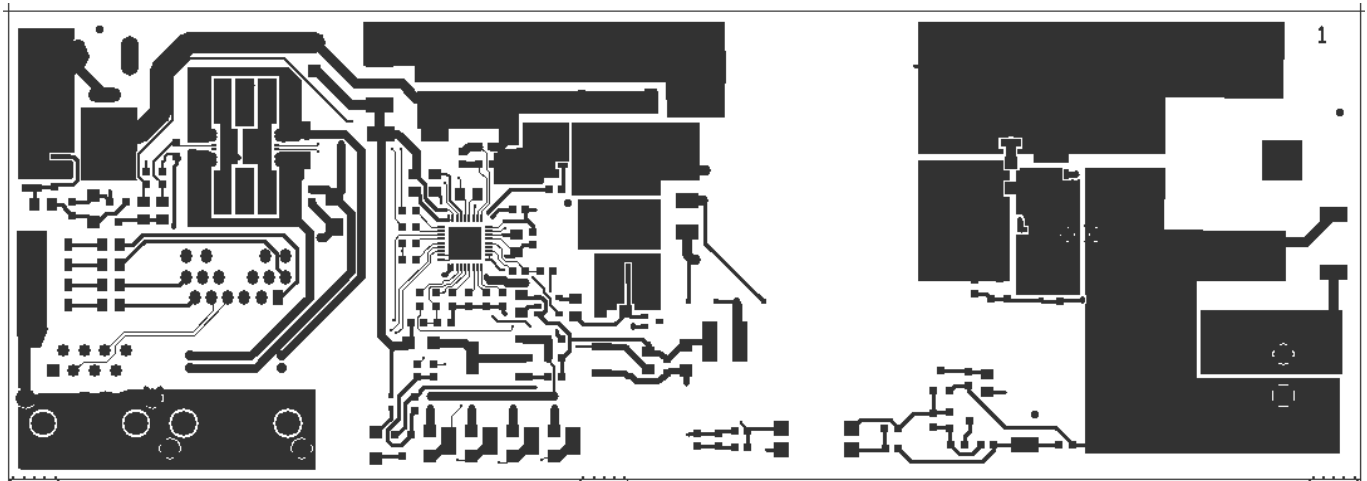
Figure 16: Top Layer
