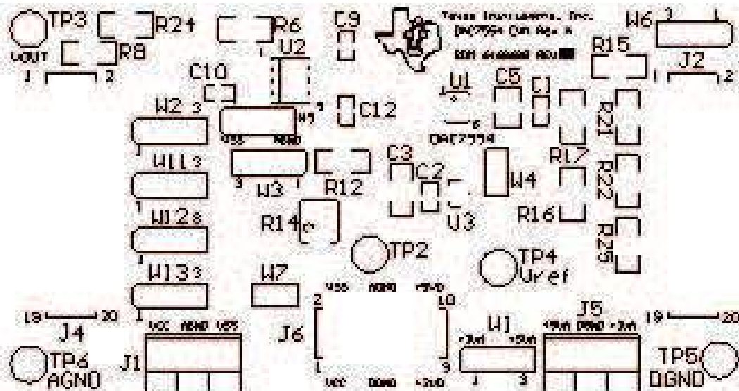
DAC7554 REV A LAYER SILKSCREEN TOP
