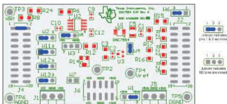
Figure 7. Factory Default Jumper Setting
