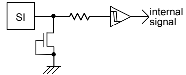
Figure 54. SI input equivalent circuit
