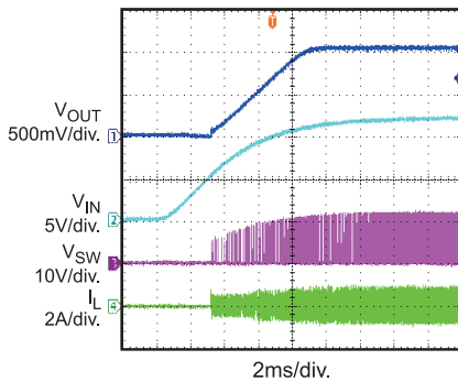
Start-Up Through VIN I_{OUT} = 0A , PWM Mode
