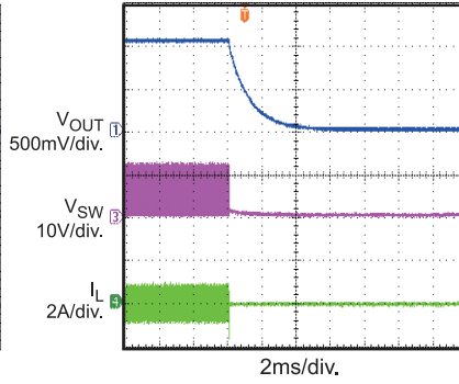
Thermal Shutdown
