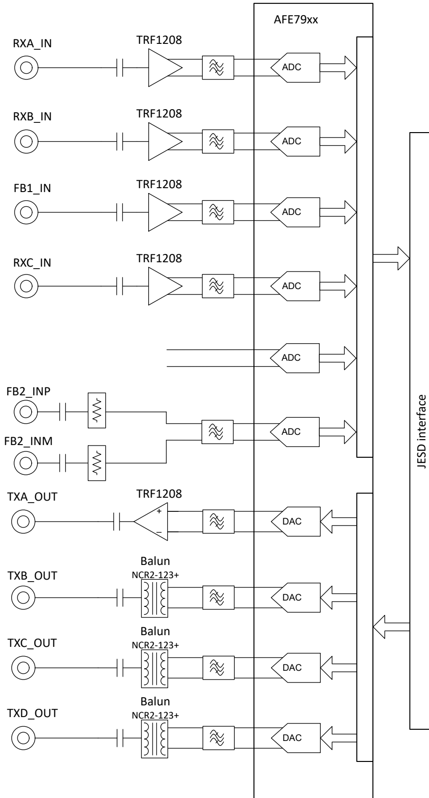
Figure 1-4. AFE79 + TRF1208 EVM Block Diagram
