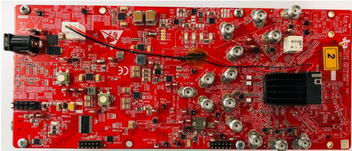
Figure 1-1. TRF1208-AFE7950-EVM Top View
