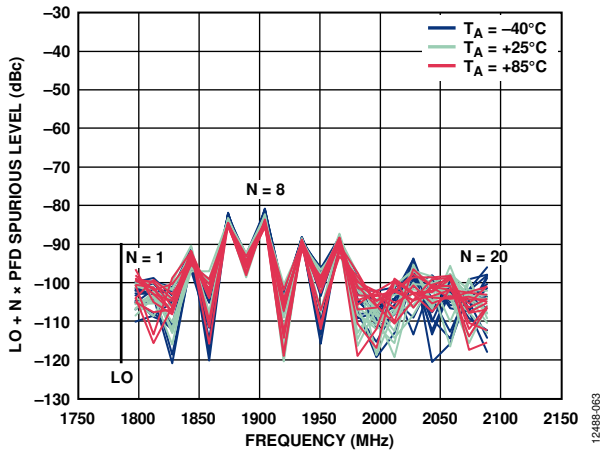
Figure 60. PFD Spurious Emissions on Modulator Output, f_{LO} + N \times f_{PFD} ; f_{LO} = 1781.76 \text{ MHz} , RF_{OUT} \approx 4 \text{ dBm} at 25^\circ\text{C} , f_{REF} = 61.44 \text{ MHz} at 4 \text{ dBm} , f_{PFD} = 15.36 \text{ MHz} , Integer PLL Mode
