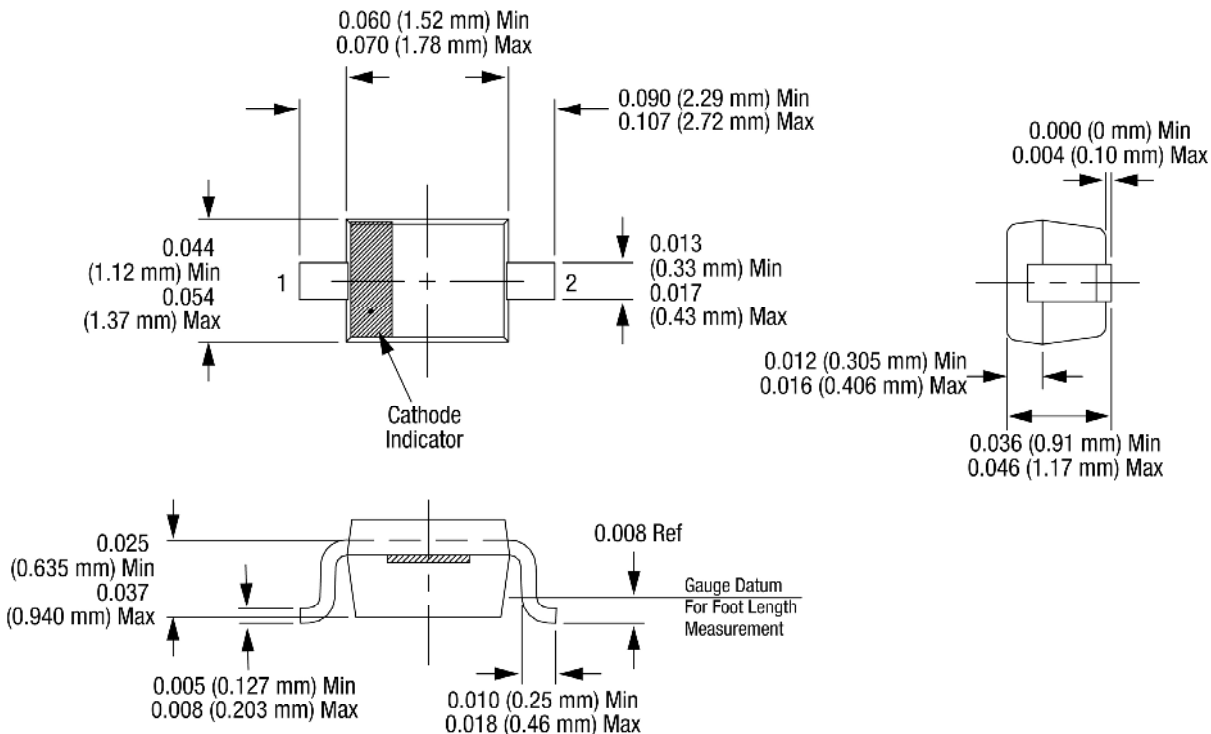
Figure 11. SOD-323 Package Dimension Drawing
