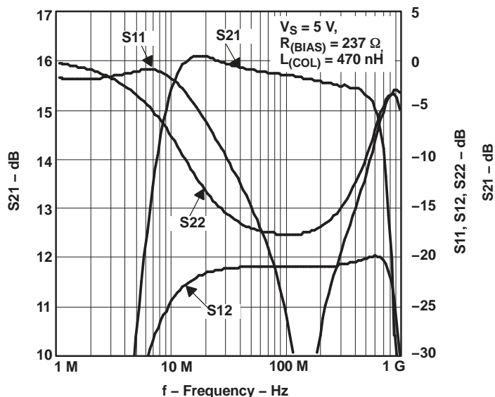
Figure 20. S-Parameters of THS9000 mounted on the standard EVM with V_S = 5\text{ V} , R_{(BIAS)} = 237\ \Omega , and L_{(COL)} = 470\text{ nH}
