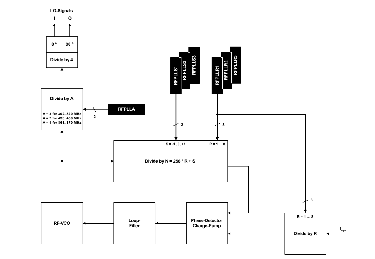
Figure 16 RF PLL
