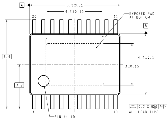
DIMENSIONS ARE IN MILLIMETERS DIMENSIONS IN ( ) FOR REFERENCE ONLY
