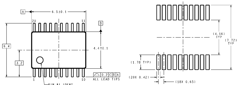
LAND PATTERN RECOMMENDATION
