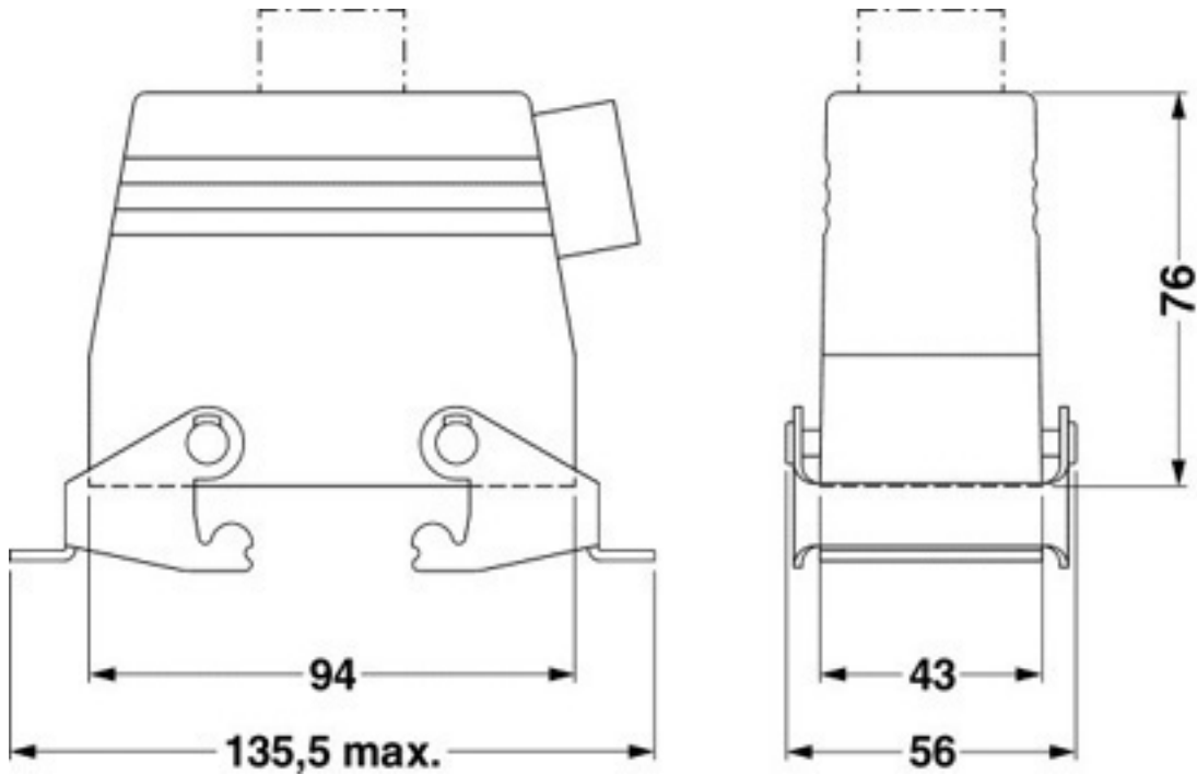
Dimensioned drawing
