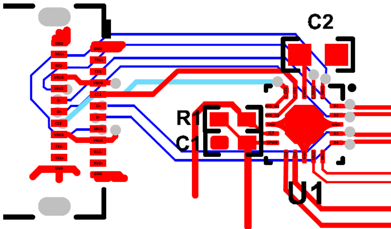
Figure 34. TPD8S300A Typical Layout
