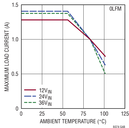
Derating, V_{OUT} = -3.3V , DC2753A Demo Board
