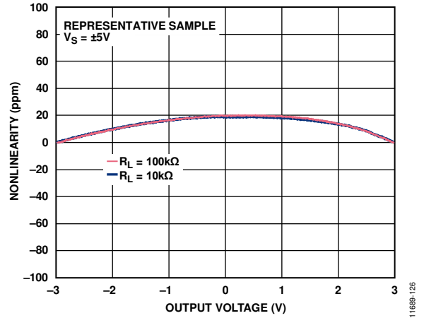
Figure 26. Nonlinearity, V_S = \pm 5\text{ V}
