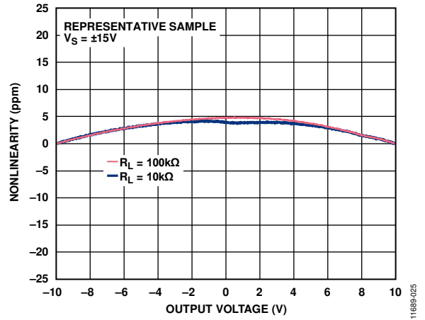
Figure 25. Nonlinearity, V_S = \pm 15\text{ V}
