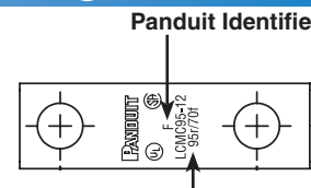
Rigid and Flexible Stranded Conductor Sizes Marked on Part
