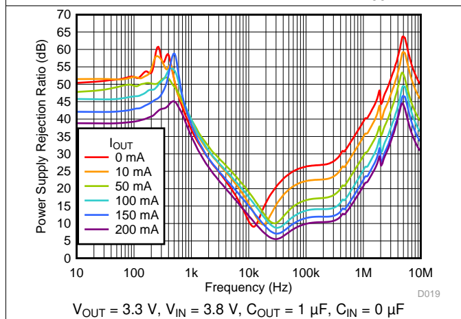
Figure 41. PSRR vs Frequency and I_{OUT}
