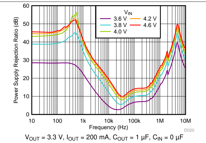
Figure 38. PSRR vs Frequency and V_{IN}
