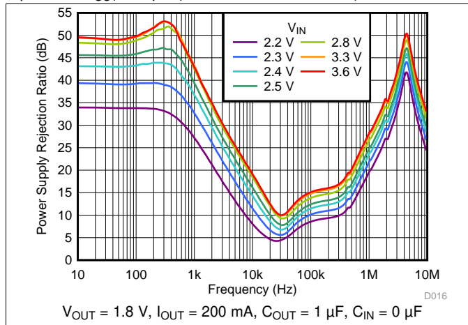
Figure 37. PSRR vs Frequency and V_{IN}
