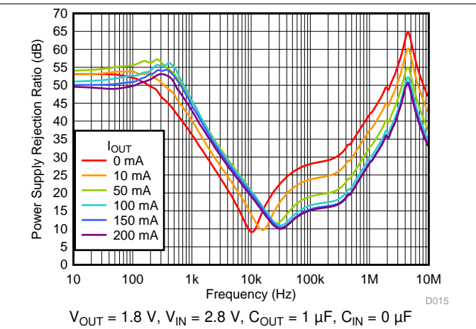
Figure 40. PSRR vs Frequency and I_{OUT}
