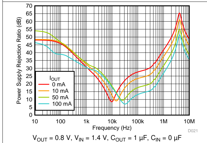
Figure 39. PSRR vs Frequency and I_{OUT}
