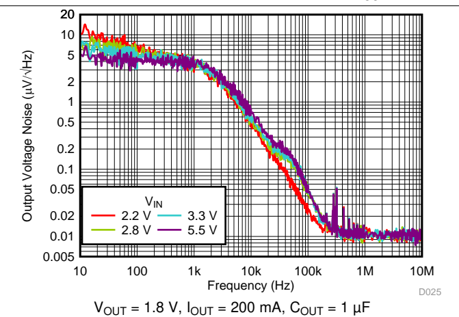
Figure 42. Output Noise vs Frequency and V_{IN}
