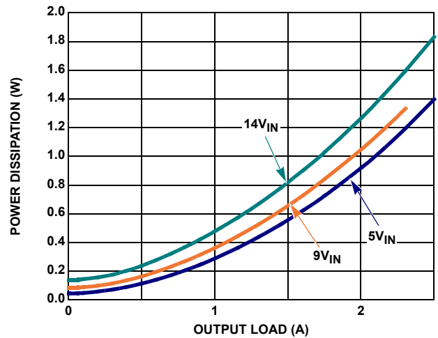
FIGURE 14. POWER DISSIPATION vs LOAD ( V_{OUT} = 0.6V, 500kHz )
