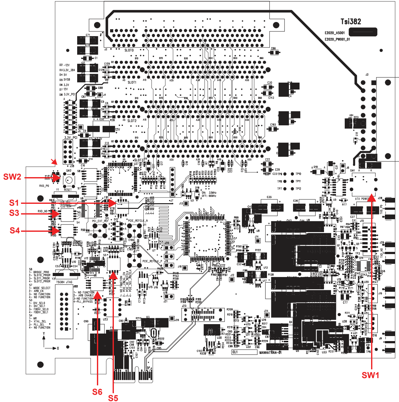
Figure 6: Switch Locations
