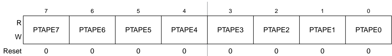
Figure 6-7. Pullup Enable for Port A (PTAPE)
