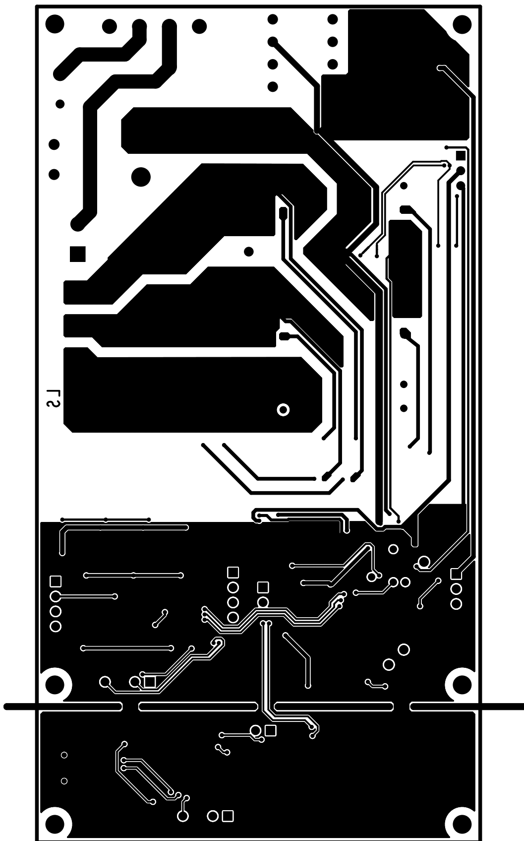
Figure 8. EVSPIN32F06021s – Layout (bottom layer)
