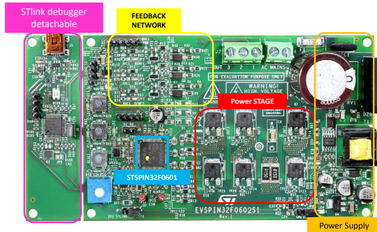
Figure 5. EVSPIN32F06021s – Board functions description
