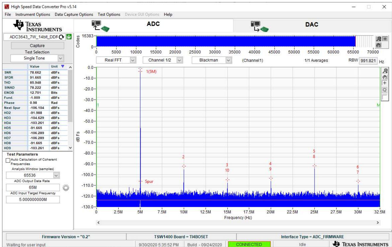
Figure 4-5. Bypass Mode Capture
