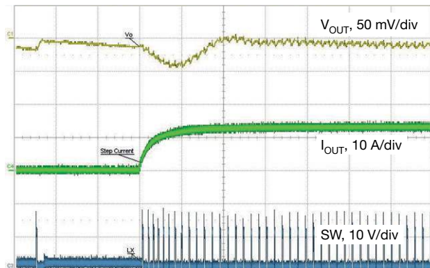
Fig. 31 - Load Step, 0.1 A to 12 A, 1 A/ \mu s, t = 10\text{ }\mu s/div Skip Mode Enabled
