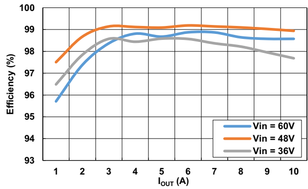
Figure 29. Efficiency, 48V
