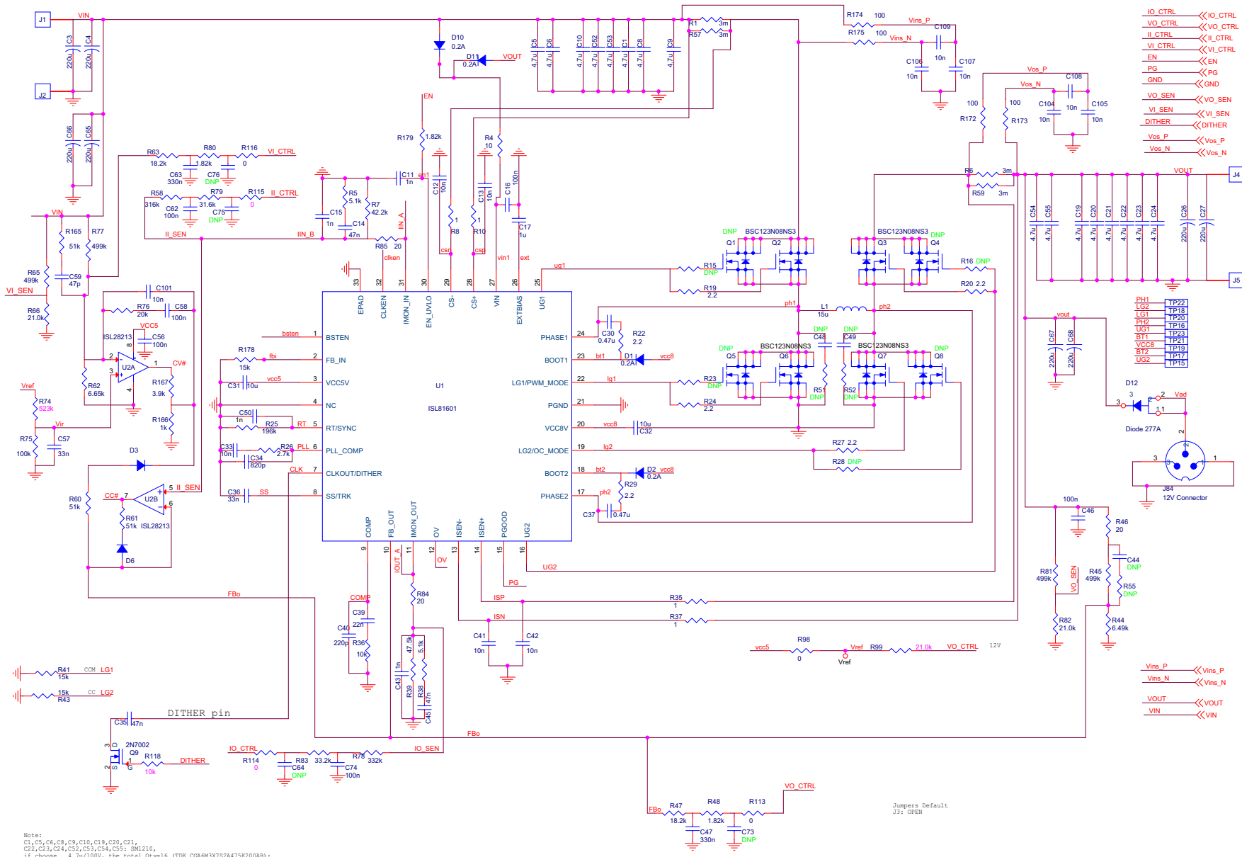
Figure 20. ISL81601 Schematic
