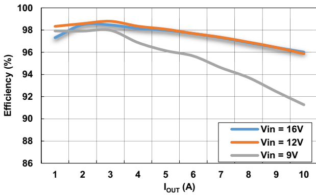
Figure 28. Efficiency, 12V
