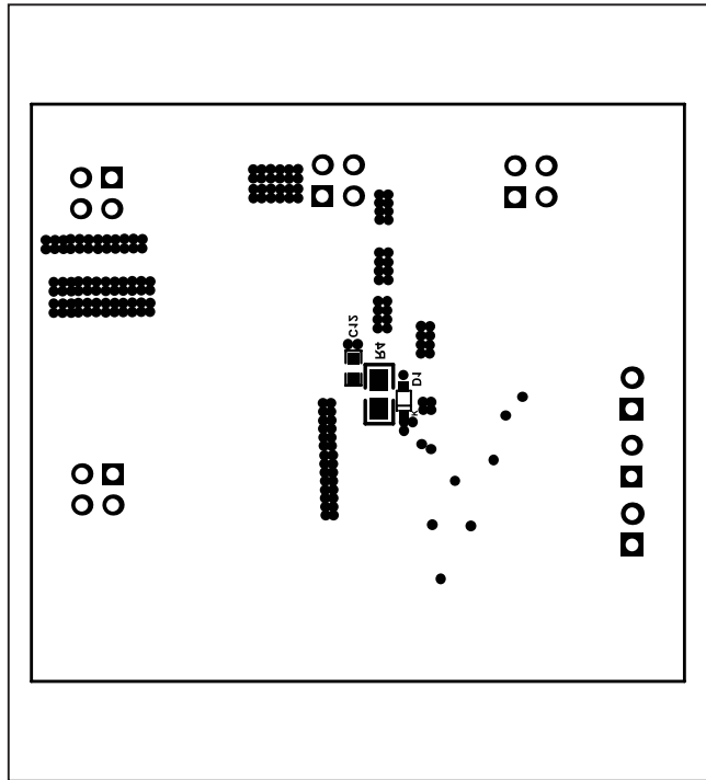
Figure 7. MAX15066 EV Kit Component Placement Guide—Solder Side
