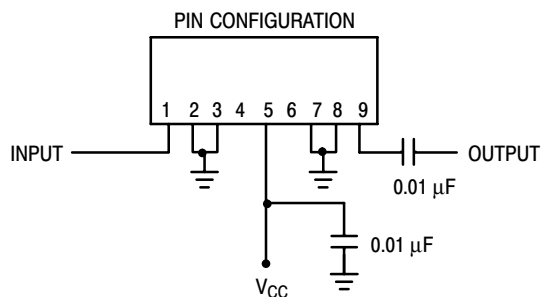
Figure 1. External Connections
